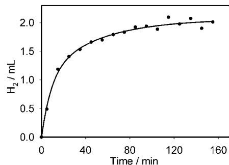
Figure 2. Photocatalytic H 2 production over time in 1.0 M acetate buffer at pH 4.0 with 0.1 M ascorbic acid, 0.5 mM [Ru(bpy) 3 ] 2+ , and 5.0 μM 2 at 22 °C.
